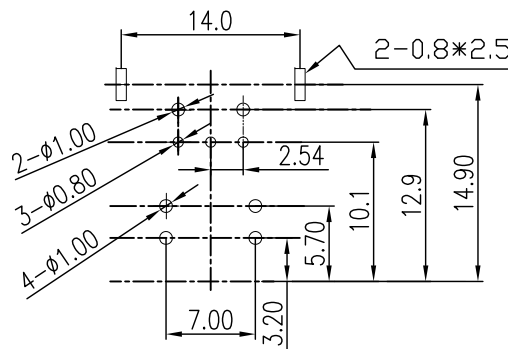
Recommended P.C.Board hole
