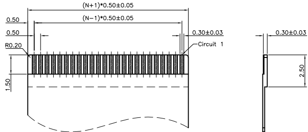
RECOMMENDED FPC/FFC DIMENSION
