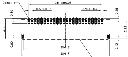
RECOMMENDED P.C.B PATTERN LAYOUT
