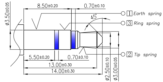
Matching Plug
