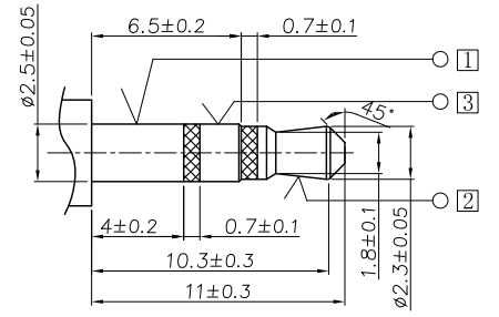
Matching Plug
