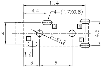
RECOMMENDED P.C.B LAYOUT TOP VIEW (TOLRANCE:±0.05)
