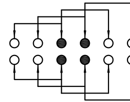
SCHEMATIC (SHORTING)
