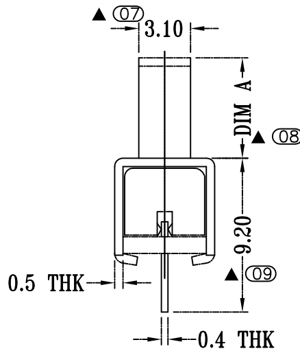
SCHEMATIC (NON-SHORTING)
